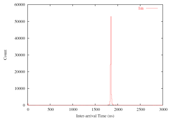
Figure 11: The Closer Look at Inter-arrival Distribution of Large Packet Train (1 meter)
